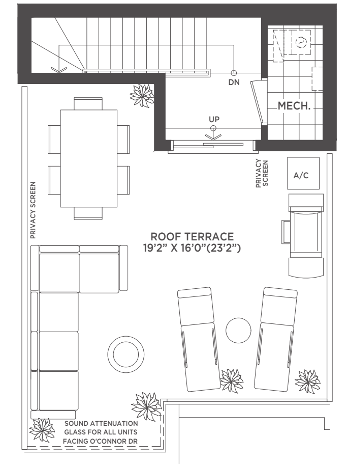
ROOFTOP LEVEL
