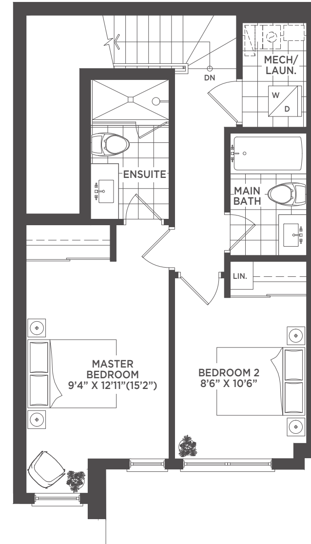
UPPER LEVEL
